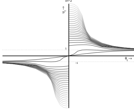
Figure 1.4: Dual control solution with end cost \phi(x) = x^2 and path cost \int_t^{t_f} dt' \frac{1}{2} u(t')^2 and \nu = 0.5 . Plot shows the deviation of the control from the certain case: u_t(x, \theta)/u_t(x, \bar{\theta} = \pm\infty) as a function of \theta for different values of t . The curves with the larger values are for larger times-to-go.
