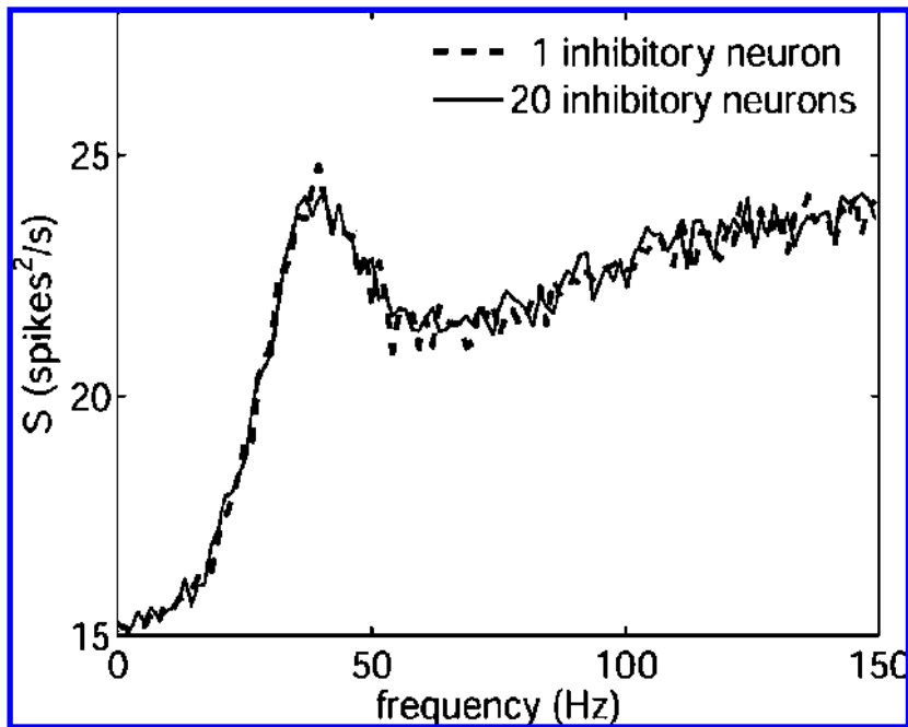
Figure 3: Spike train power spectra of an excitatory neuron for spatially correlated input when inhibition is provided by a single LIF neuron (dashed line) or a population of 20 inhibitory LIF neurons (solid line). All other parameters as in Figure 2.
