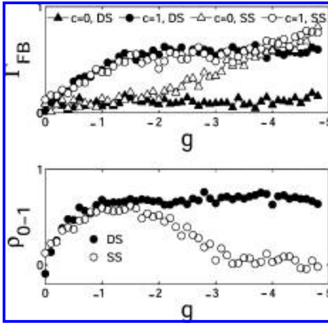
Figure 7: (Top) Power \Gamma_{FB} = \Gamma_{30,50} - \Gamma_{2,22} near the resonance peak (30–50 Hz) relative to that in the frequency range between 2 and 22 Hz in the presence of correlated ( c = 1 ; circles) and uncorrelated ( c = 0 ; triangles) input, with static synapses (SS; open symbols) and dynamic synapses (DS; filled symbols). (Bottom) Ability to discriminate correlated and uncorrelated input \rho_{0-1} (see equation 3.2) for static (SS, open symbols) and dynamic (DS, closed symbols) synapses as a function of the inhibitory gain.
