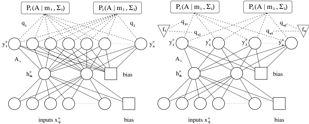
Figure 2: The task clustering (left) and task gating model (right). In task clustering the task-dependent weights \mathbf{A}_i are supposed to be drawn from a weighted sum of Gaussians, where the weights q_\alpha are equal for all tasks. In task gating these weights become task-dependent and the value for q_{i\alpha} depends on the task-specific feature vector \mathbf{f}_i .
