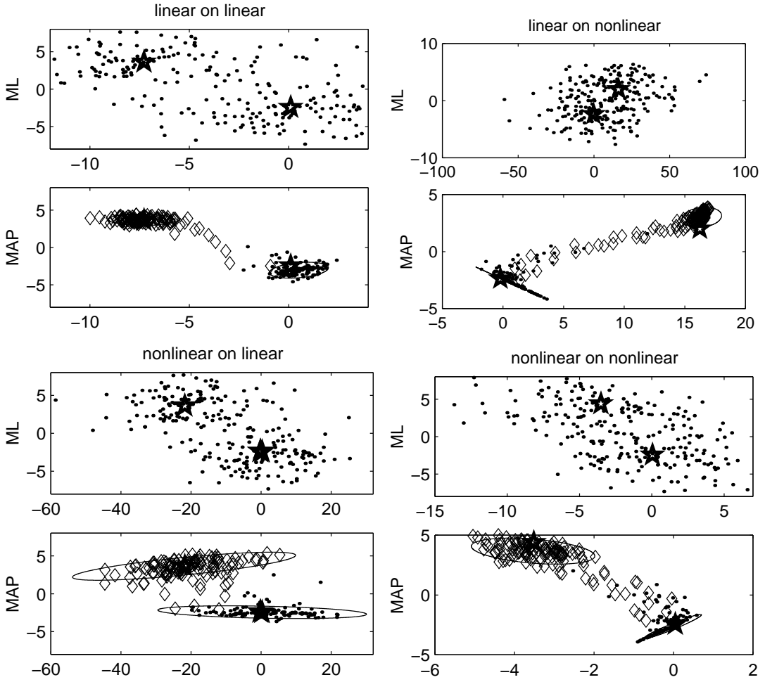
Figure 3: Maximum likelihood (upper panels, marked ML) and maximum a posteriori (lower panels, marked MAP) values for the model parameters A in the artificial data paradigm. In each panel, the horizontal axis corresponds to the hidden-to-output weight, the vertical axis to the bias. The 95% confidence intervals for the two estimated priors are plotted in the lower panels. From left to right and up to down, the panels show the results for the linear model on the linear data, the same model on the nonlinear data, the nonlinear model on the linear data and on the nonlinear data. The means m_\alpha used for generation of the data sets (corrected for the difference between the true and estimated hidden unit activity) are depicted by stars in the 8 panels.
